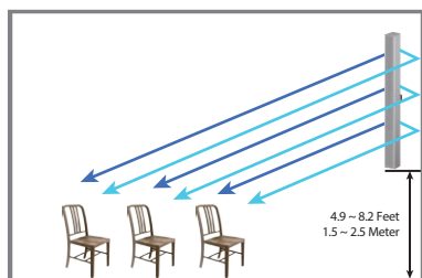
Sound Field of SMARTVOX-II-30/60 Line Array (figure 2)
